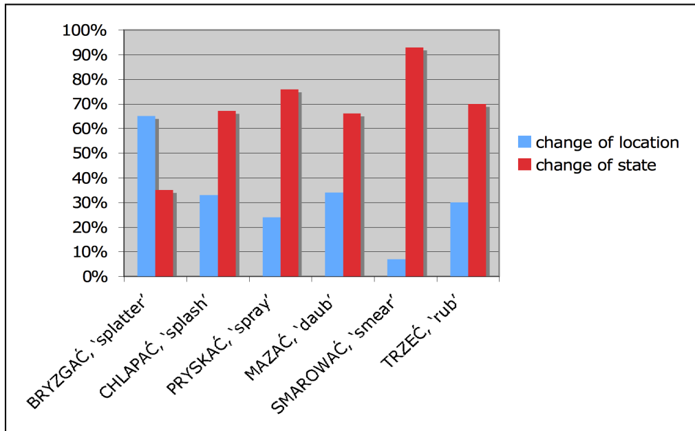
Diagram 1: Distribution of manner verbs in the locative alternation variants in Polish
