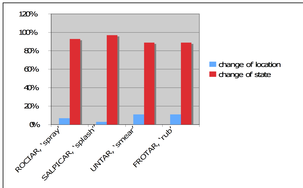
Diagram 2: Distribution of manner verbs in the locative alternation variants in Spanish
